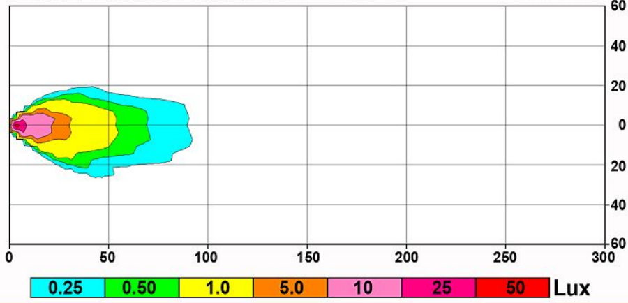
Flood Beam Pattern (1.0m high, -0°)
