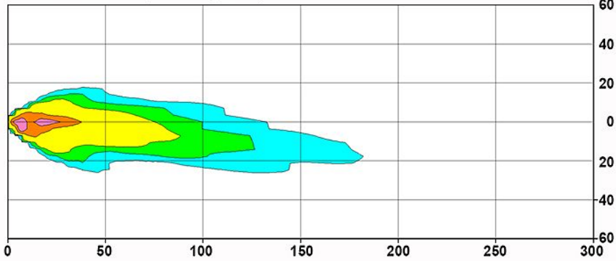
Low Beam (1.0m high, -0°)
