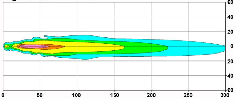
High Beam (1.0m high, -0°)
