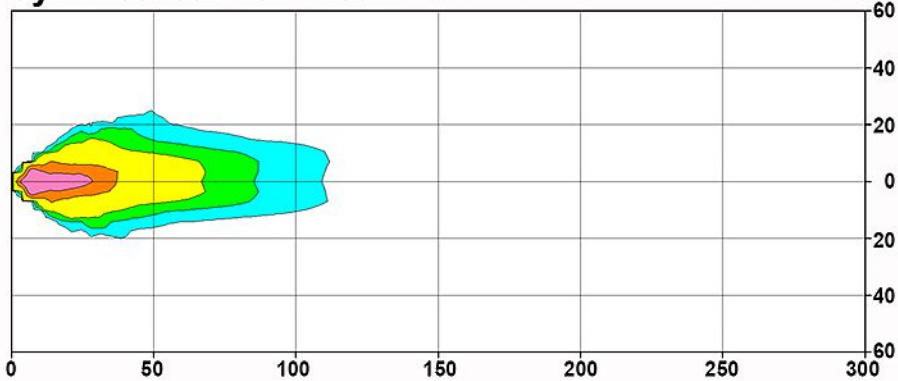
Symmetrical Low Beam (1.0m high, -0°)
